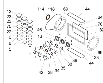
KIT 2150 (STD)
