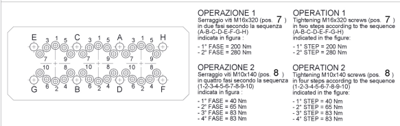
SERRAGGIO VITI CAMICIE E TESTATA TIGHTENING SHELL AND HEAD SCREWS
